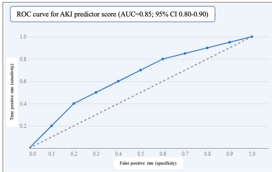
Figure 2. ROC curve for AKI predictor score.
